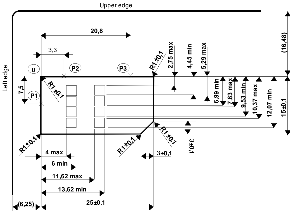
Figure 4.1: Plug-in UICC
