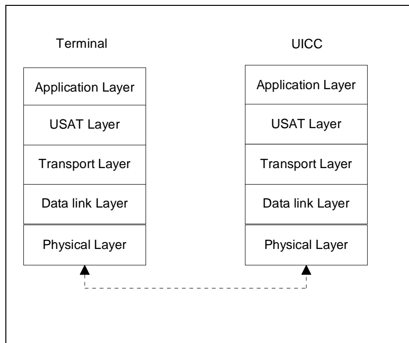
Figure 7.1: Layers
