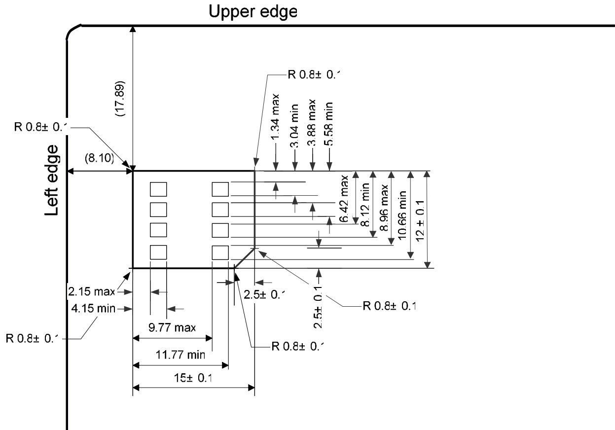
Figure 4.2: Mini-UICC
