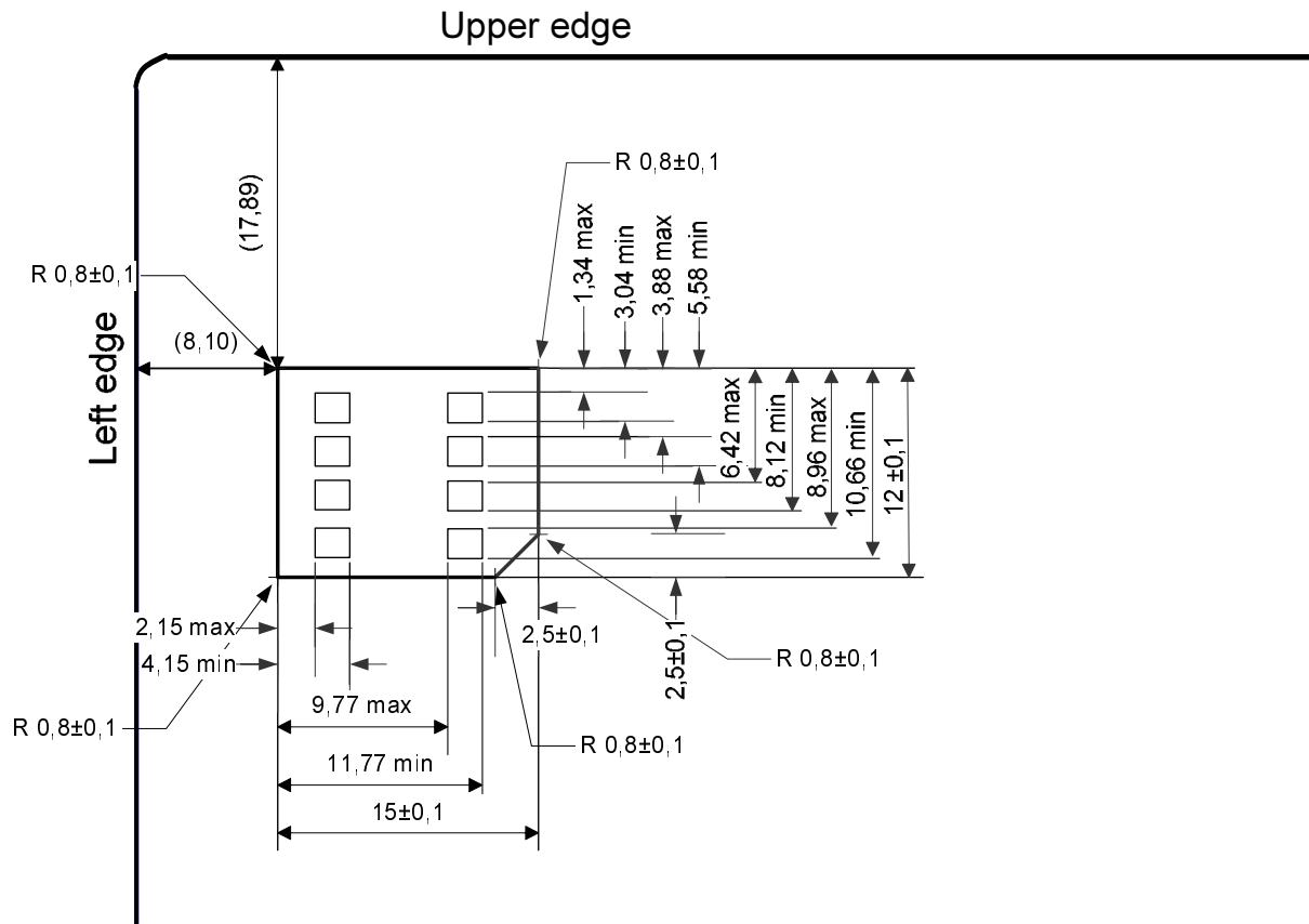
Figure 4.2: Mini-UICC
