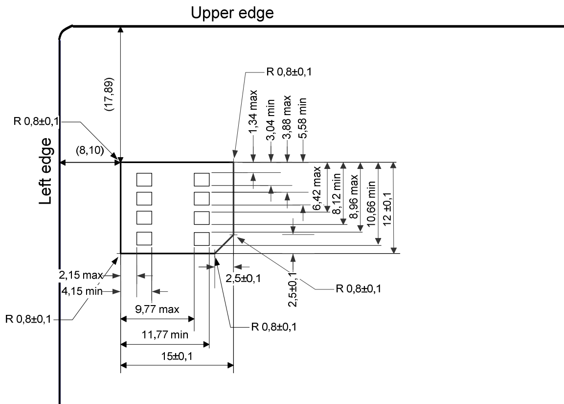
Figure 4.2: Mini-UICC
