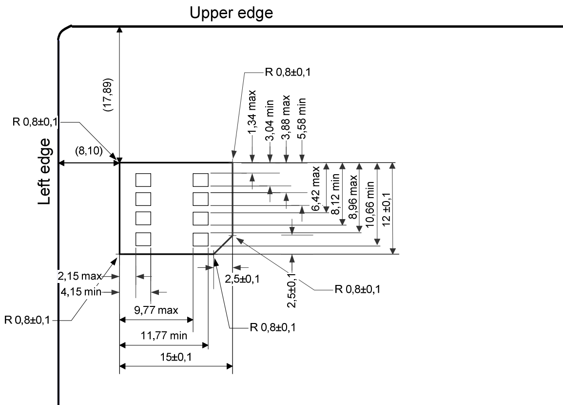
Figure 4.2: Mini-UICC
