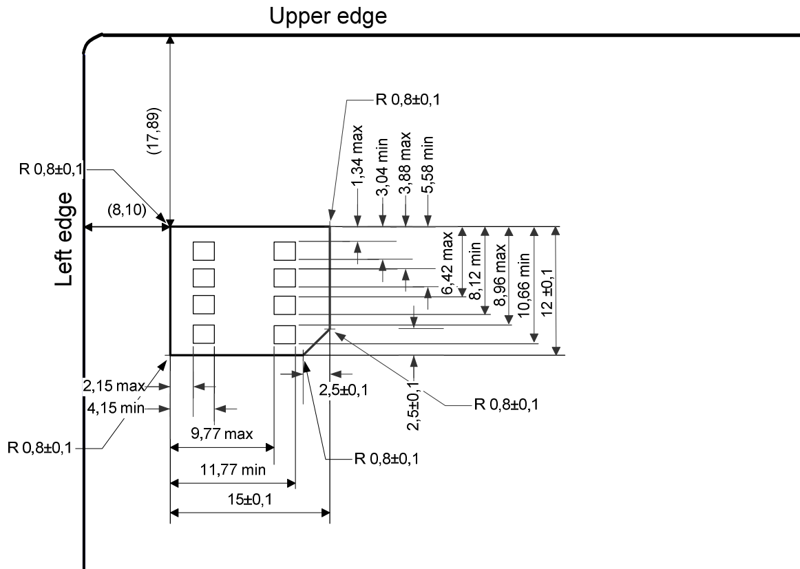
Figure 4.2: Mini-UICC
