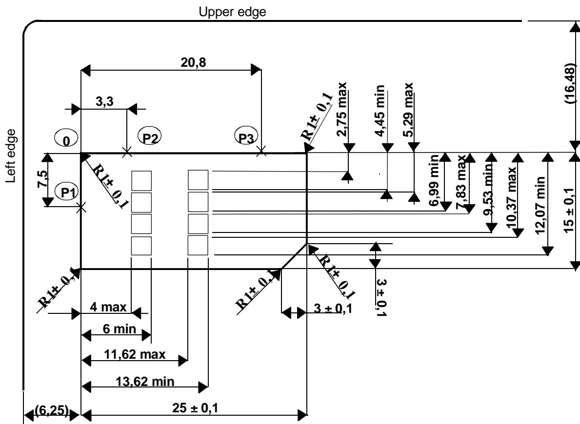
Figure 4.1: Plug-in UICC
