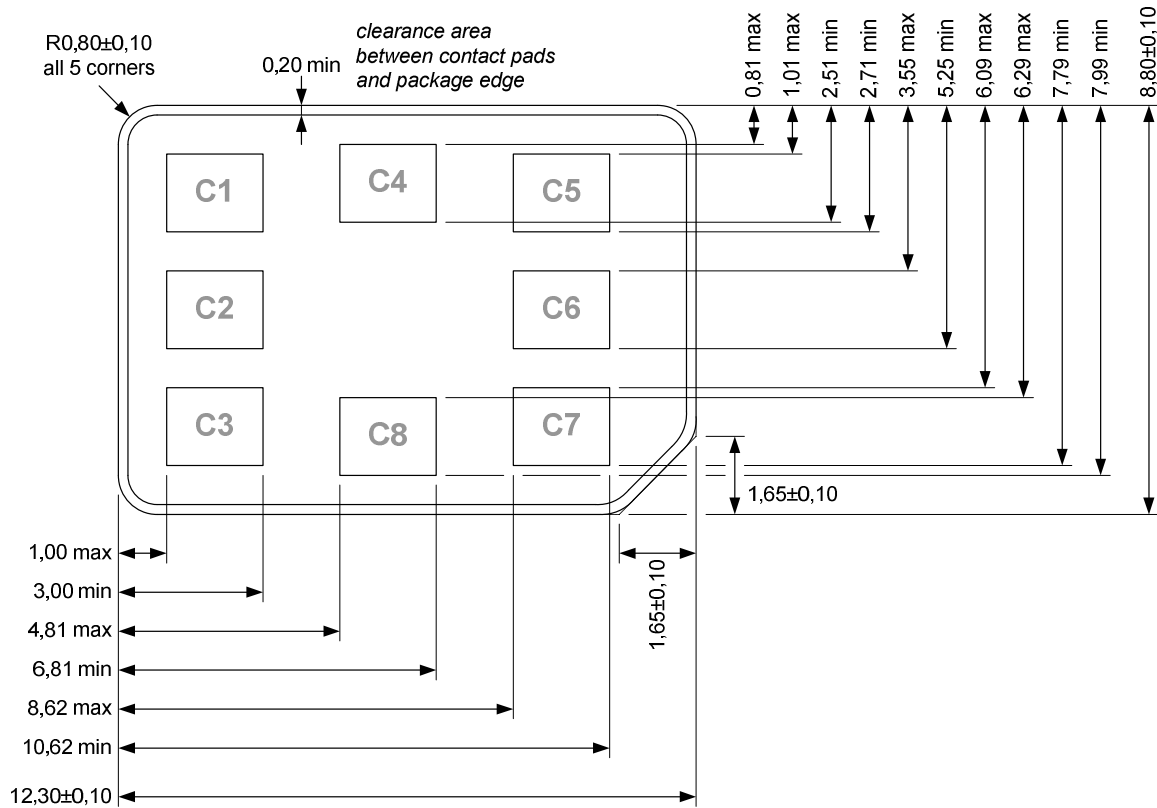
Figure 4.3: 4FF
