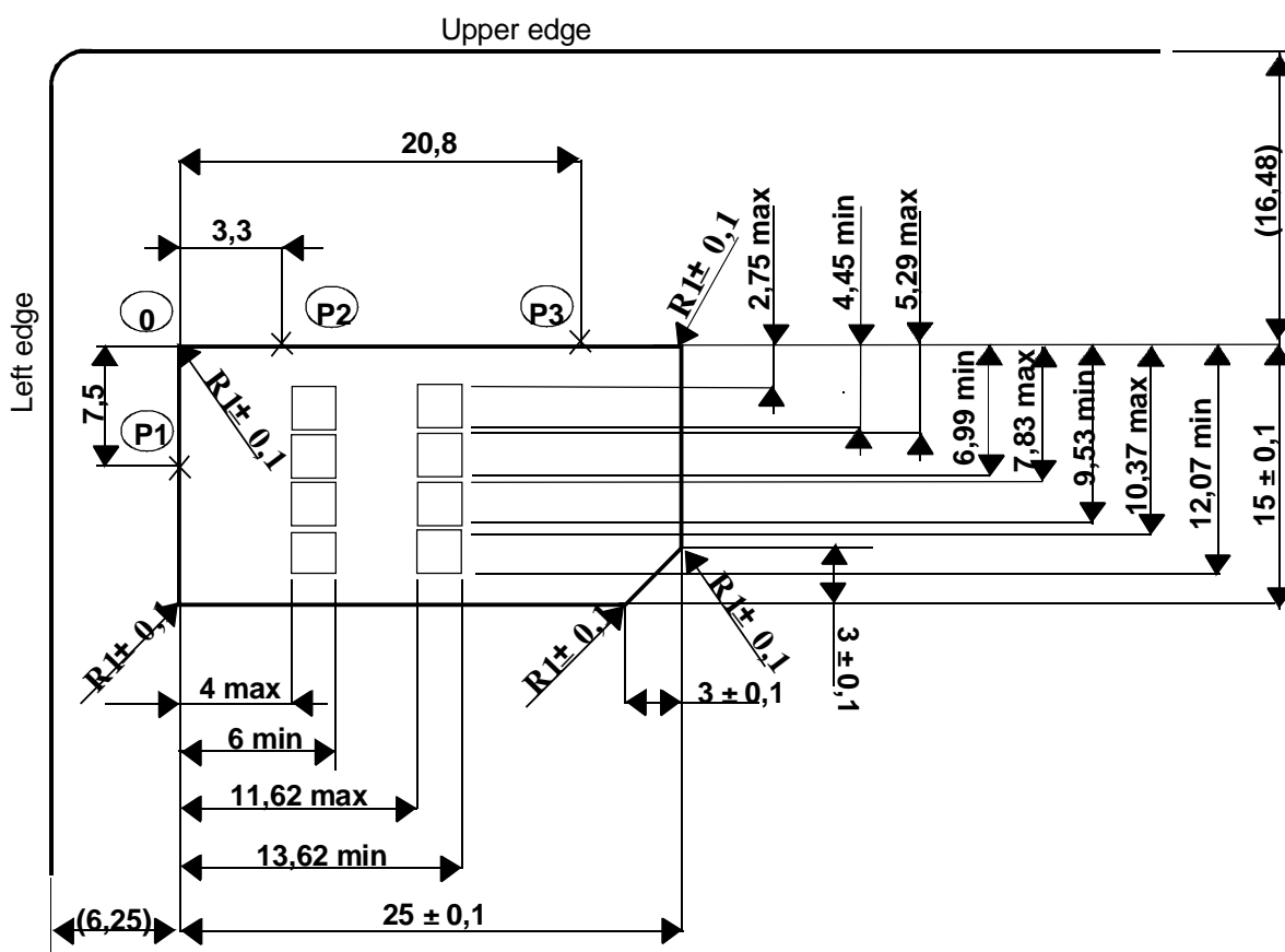
Figure 4.1: Plug-in UICC
